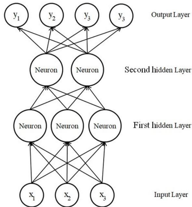
Figure 3: Feed-forward neural network with two hidden layers; Source: Author's own representation
