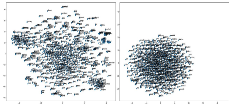
Figure 20: TT-SNE projection of word vectors for the TREC vocabulary. On the left vectors from GloVe. On the right random initialization of dimension 300; Source: Author’s own representation
