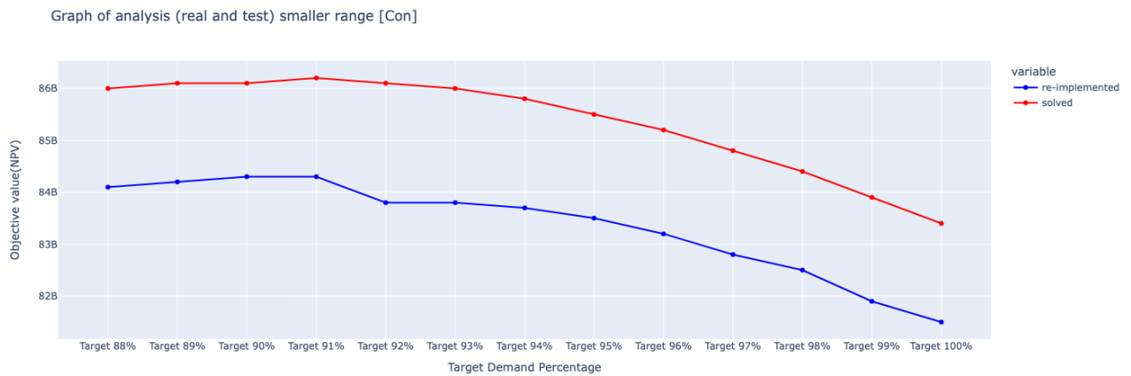
Figure A.2 Real and Test Gap Analysis (88% - 100%) [CON]
